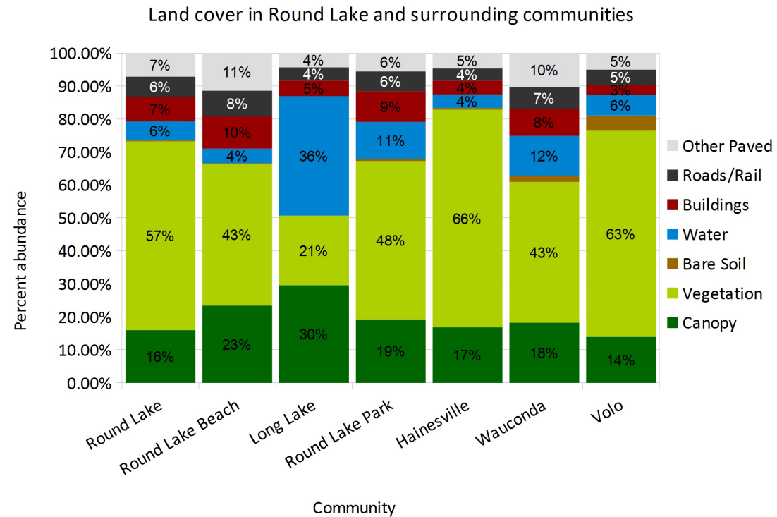
Figure 7: Comparison of land cover of Round Lake and its neighbors.
