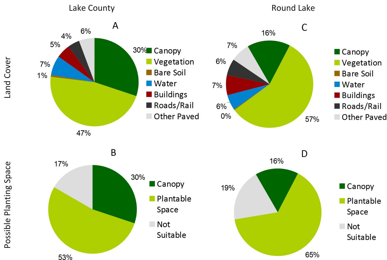
Fig 2: Lake County's current land cover (A), including 30% canopy cover. An additional 53% of the county is suitable for planting (B). Round Lake currently has 16% canopy cover (C), and 65% of the land cover could potentially be converted to canopy (D).
