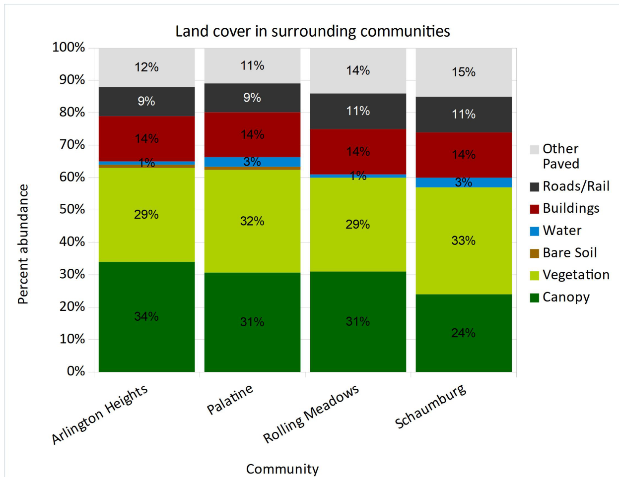
Figure 9: Comparison of land cover of Rolling Meadows and its neighbors.
