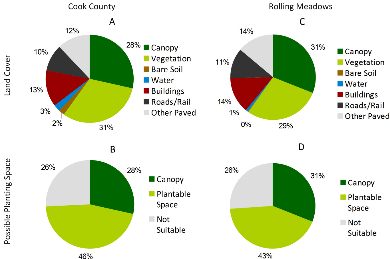
Fig 2: Cook County's current land cover (A), including 28% canopy cover. An additional 46% of the county is suitable for planting (B). Rolling Meadows currently has 31% canopy cover (C), and 43% of the land cover could potentially be converted to canopy (D).
