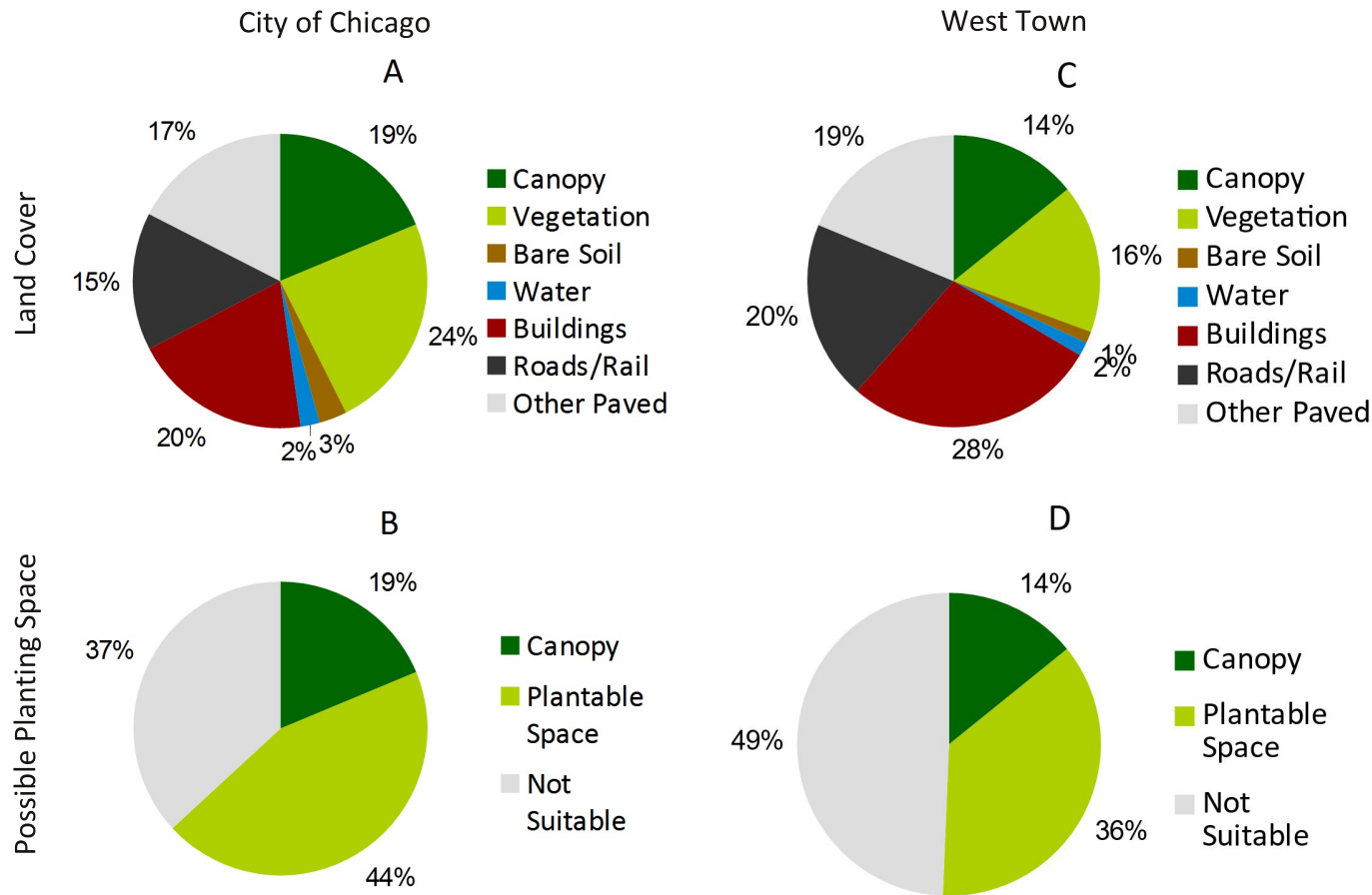
Fig 2: The City of Chicago's current land cover (A), including 19% canopy cover. An additional 44% of the county is suitable for planting (B). West Town currently has 14% canopy cover (C), and 36% of the land cover could potentially be converted to canopy (D).
