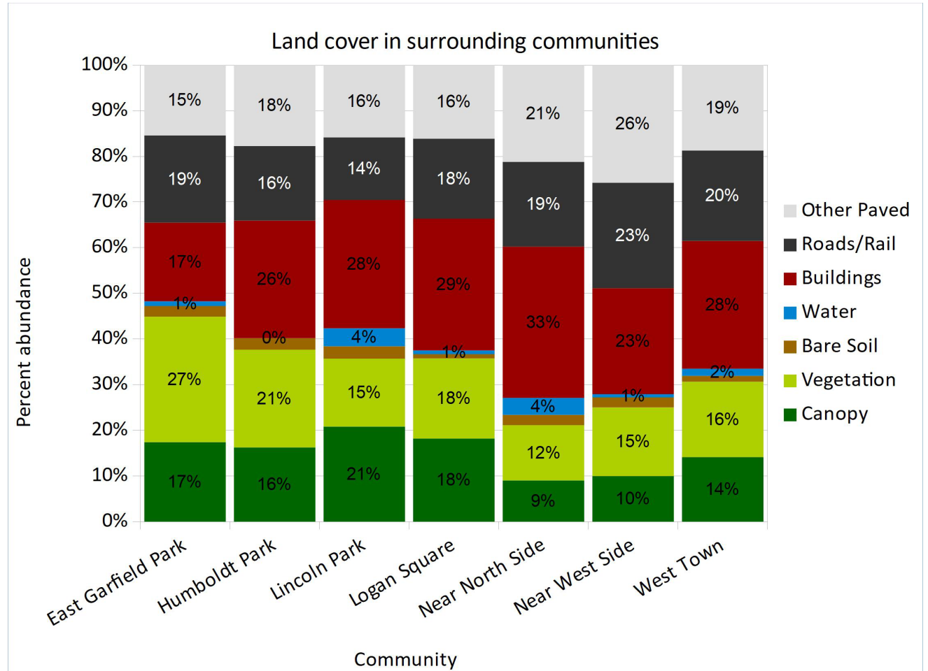
Figure 9: Comparison of land cover of West Town and its neighbors.
